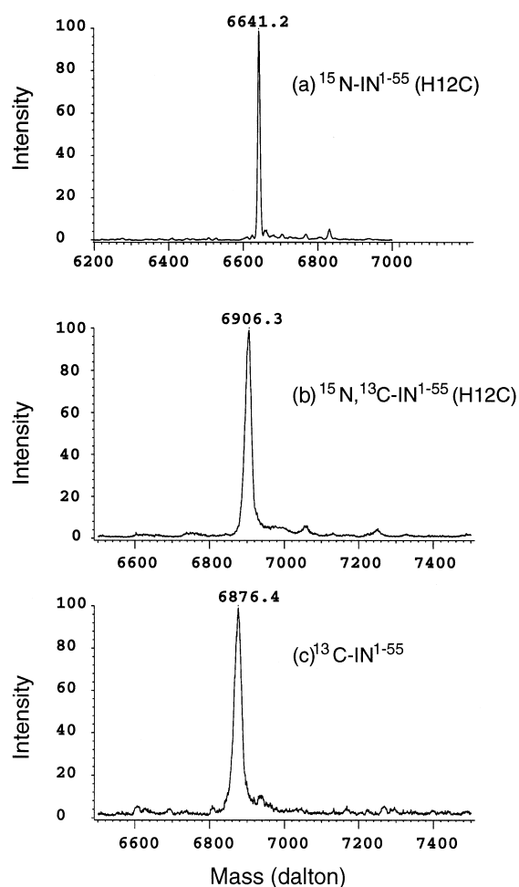
Figure 2. Mass spectra of isotopically enriched proteins: (a) 15 N-labeled IN 1-55 H12C mutant; (b) 15 N, 13 C-labeled IN 1-55 H12C mutant; and (c) wild-type 13 C-labeled IN 1-55 .
