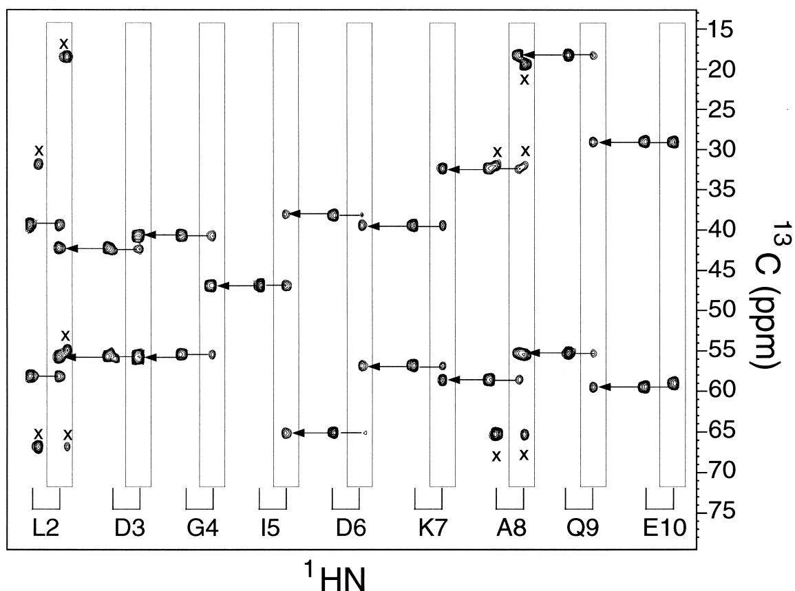
Figure 4. Strips from the 3D CBCANH (boxed) and CBCA(CO)NH triple-resonance experiments recorded at 30 °C on the ^{15}\text{N} , ^{13}\text{C} -labeled \text{IN}^{1-55}\text{H12C} mutant showing sequential connectivities for residues 2–10 of the protein. Cross peaks marked with an x arise from other residues which have their maximum intensities in an adjacent ^{15}\text{N} plane in the 3D spectrum. The spectra were recorded on a Bruker DMX500 spectrometer with 16 scans per increment, and acquisition times of 6.26, 18.38 and 63.24 ms in the t_1 , t_2 and t_3 dimensions, respectively.
