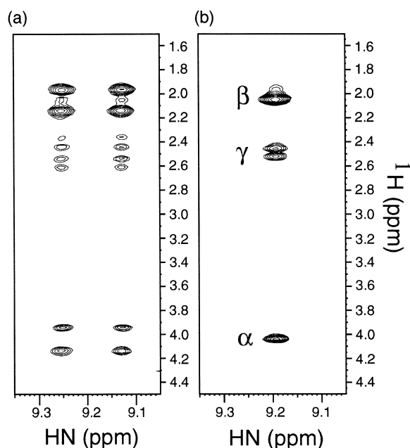
Figure 3. Selected region of the 2D ^1\text{H} - ^1\text{H} NOE spectrum (120 ms mixing time) recorded at 30 °C on the ^{15}\text{N} , ^{13}\text{C} -labeled IN ^{1-55} H12C mutant (2 mM) in water without (a) and with (b) ^{15}\text{N} and ^{13}\text{C} decoupling. The spectra were recorded on a Bruker DMX750 spectrometer and decoupling in (b) was achieved using low-power (1.5 kHz rf) Waltz decoupling for ^{15}\text{N} during the acquisition period and a ^{13}\text{C} 180° hard pulse in the middle of the t_1 evolution period for ^{13}\text{C} decoupling.
